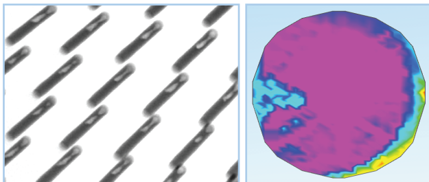
X-ray image of 10 \mu\text{m} x 100 \mu\text{m} TSVs Wafer level results
